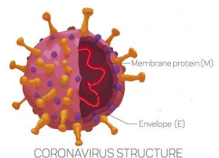
CORONAVIRUS STRUCTURE
